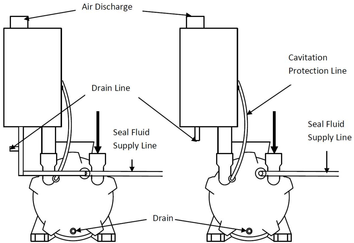
Partial Seal Recovery Configuration
