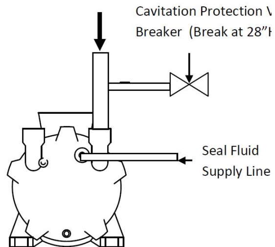
Once-Thru Configuration (w/o separator)
